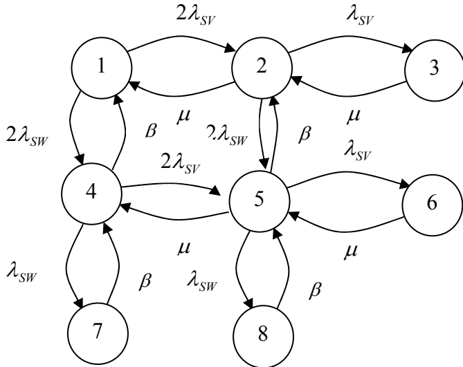
Fig. 4. CTMC for HA-OSCAR Cluster System
