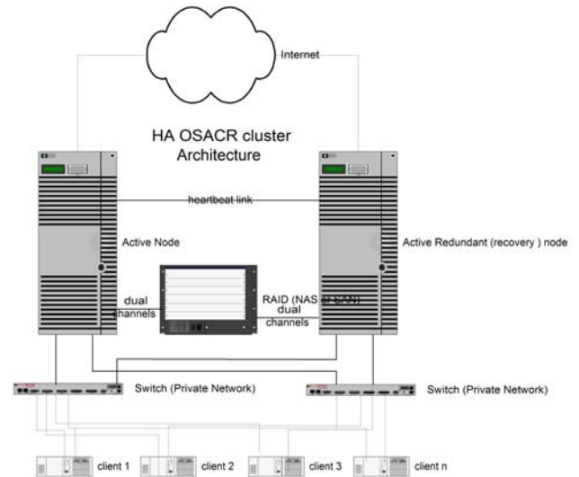
Fig. 2. A HA OSCAR Cluster System
