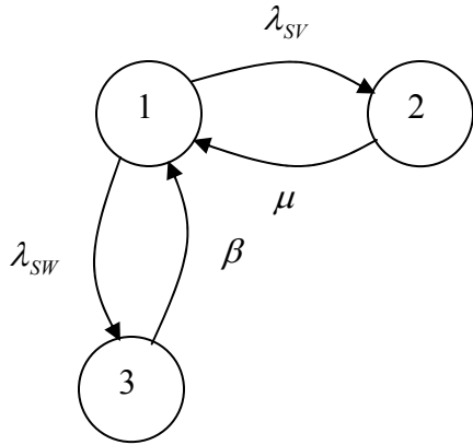
Fig. 3. CTMC for Current OSCAR Cluster System
